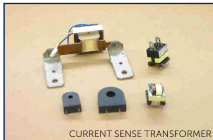
CURRENT SENSE TRANSFORMER
